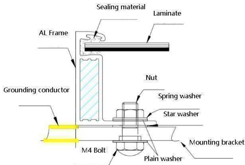
Fig. 5-8 Grounding Diagram
