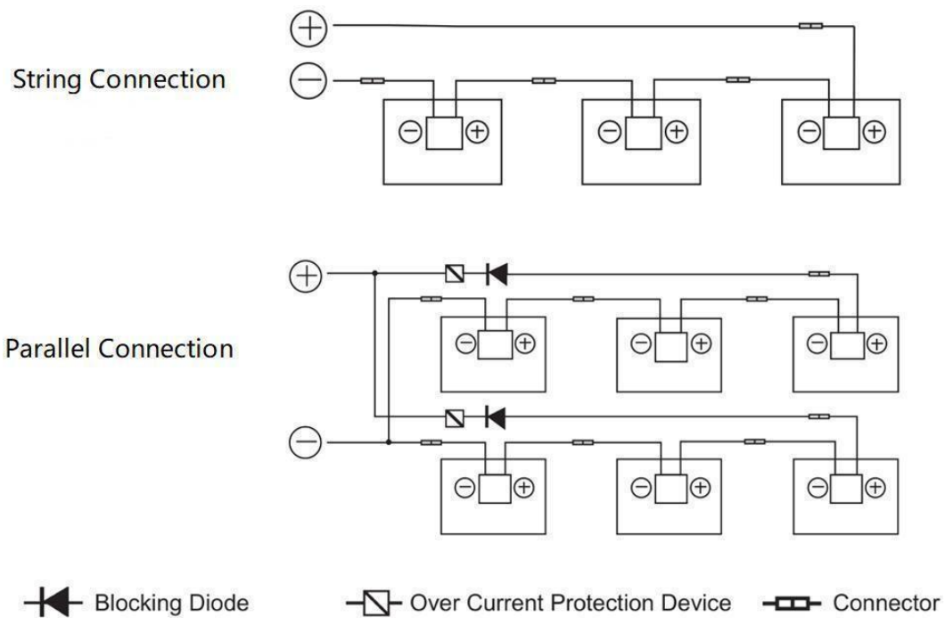
Fig. 5-7 Series Connection and Parallel Connection Circuit Diagram
