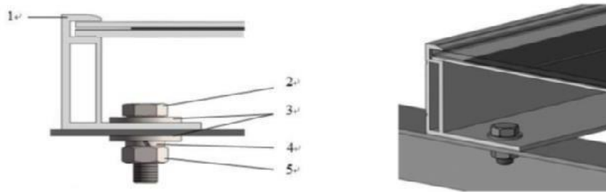
Fig.5-3 Single-glass module with frame
